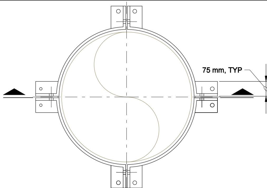
REFLECTED PLAN
